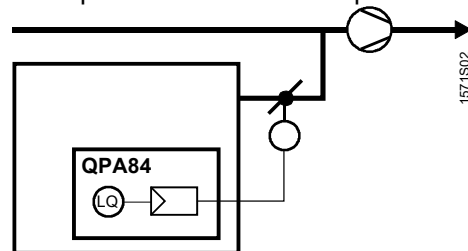
Example with extract air damper
